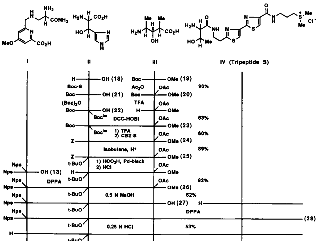
Scheme 3. Synthesis of PYML(6)-bleomycin.
